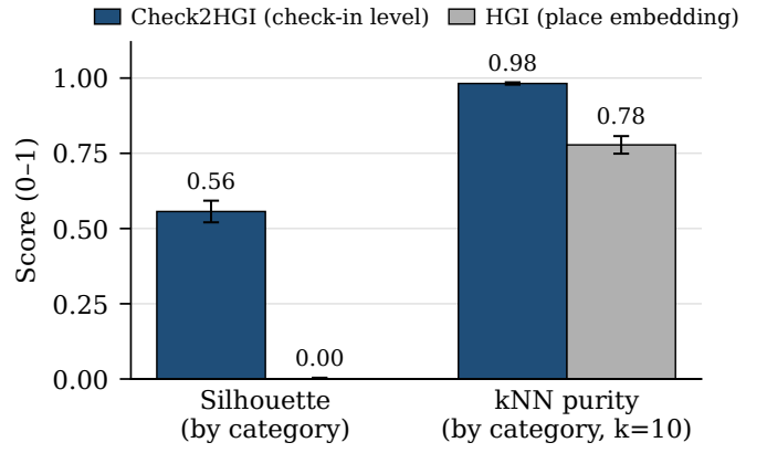
Fig. 3. Class separability of the representations, measured on the ground-truth next-category labels (cosine silhouette and leave-one-out kNN purity at k = 10 ), not on discovered clusters. The check-in-level representation cleanly separates the seven categories where the place embedding does not, which is exactly why it helps the category task and is neutral on region.
